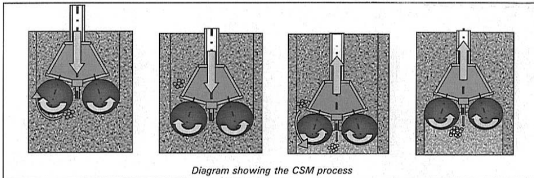
Figure 4. a) CSM layout (above) and b) rotation of cutting/mixing wheels during penetration and withdrawal (Bauer promotional information).
